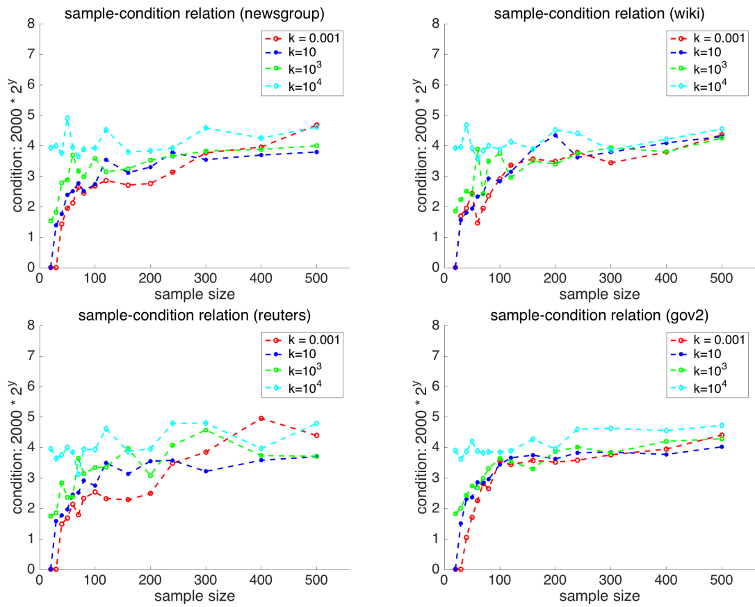
FIGURE 16: Sample-condition relation in different k - value, \beta = 10^3
